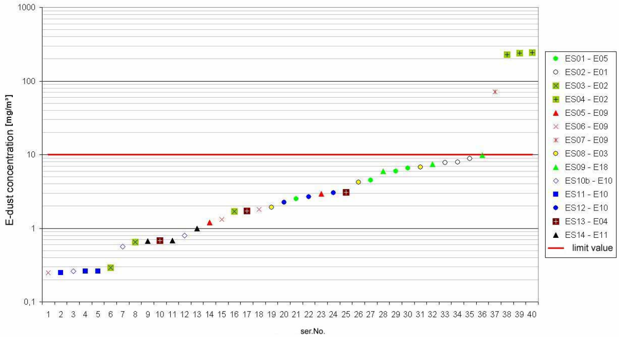
fig. 6.5.3 - 1 E-dust individual measured values for current eccentric grinders/sanders
