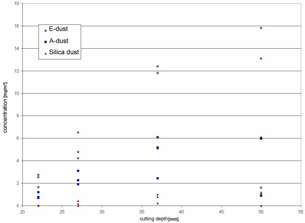
fig. 6.1.3 - 5 Influence of cutting depth on dust concentration for wall chaser MF02-E06
